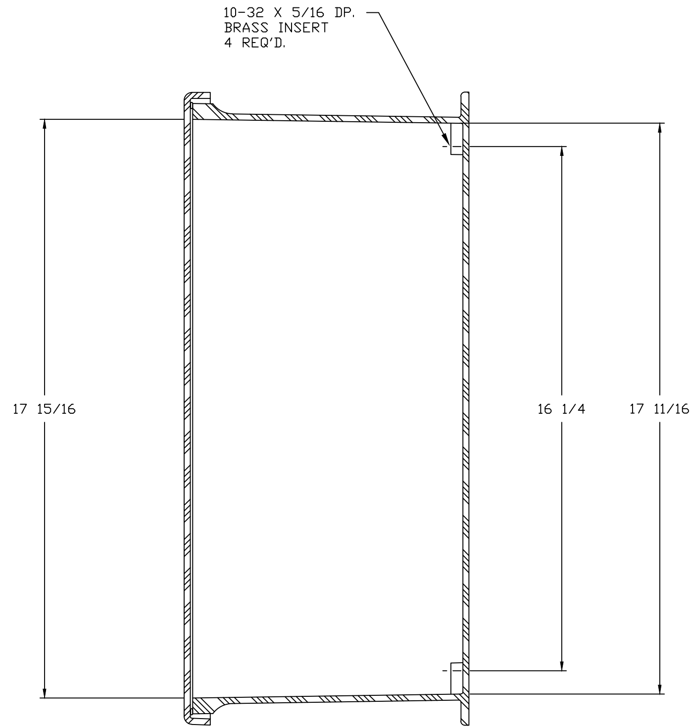
SECTION B-B
