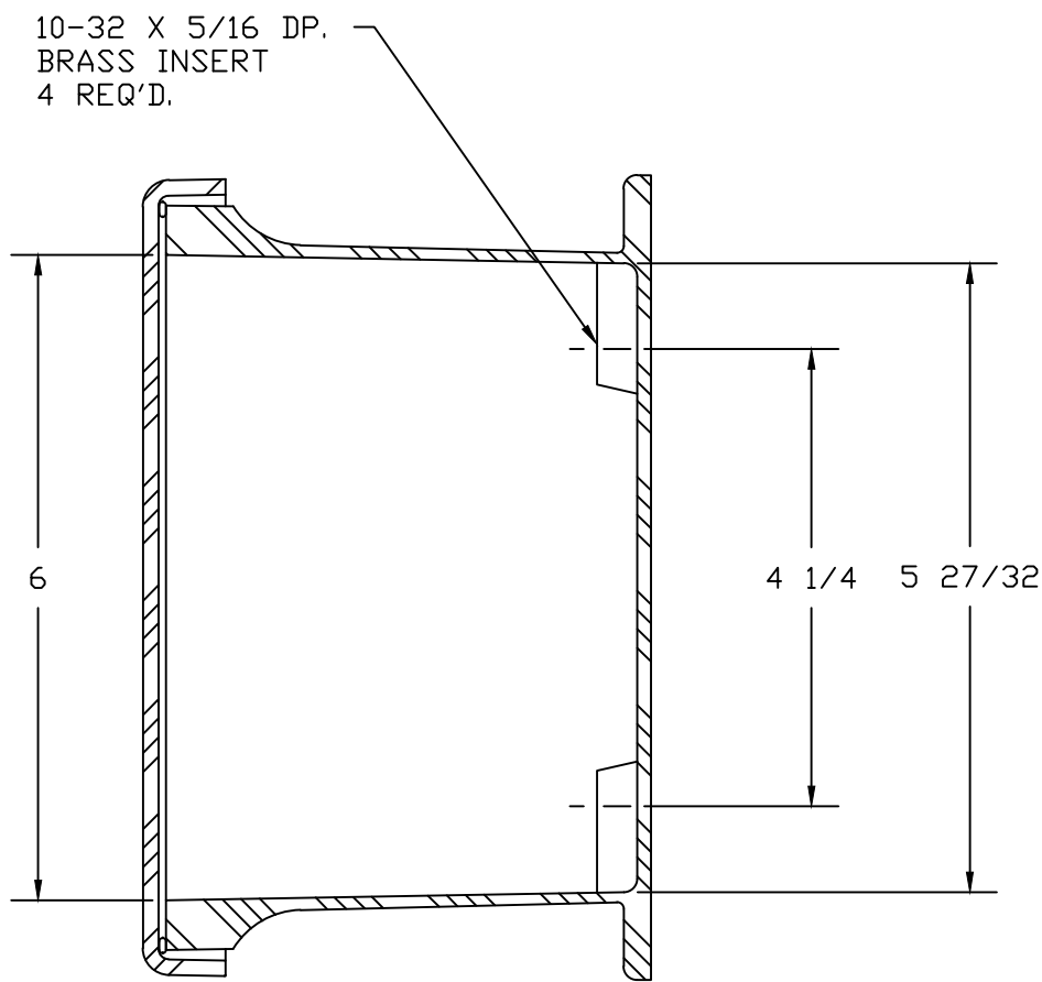
SECTION B-B
