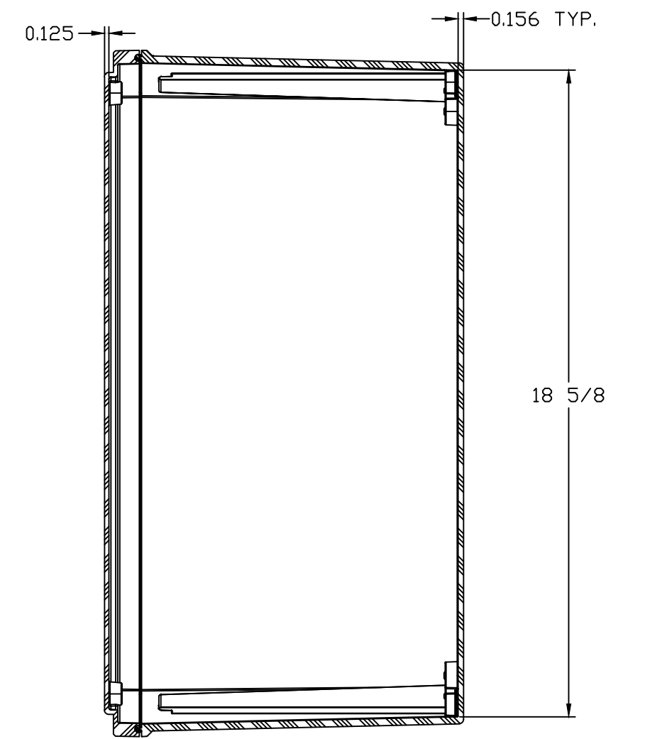
SECTION B-B
