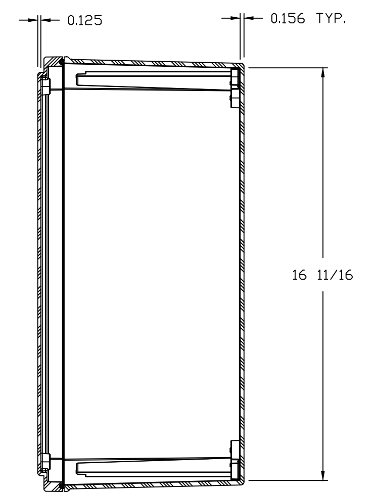
SECTION B-B
