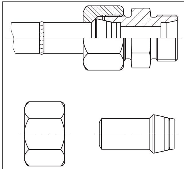
EO-Weld Nipples
