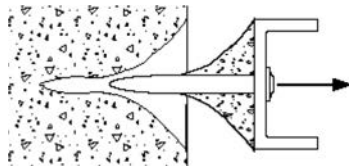
Base Material Failure Fastener Pullout
