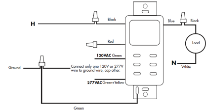
WIRING DIAGRAM: THREE-WAY INSTALLATION SS700Z
