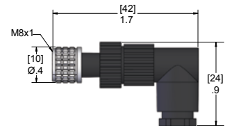
Female Plug
