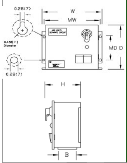
Schematic Standard w/ Grounded Secondary without Receptacle
