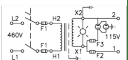
Schematic Standard w/ Grounded Secondary with Receptacle
