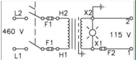
Schematic Standard w/ Grounded Secondary without Receptacle
