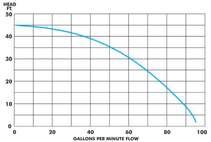
ST2010TCUL Performance Curve 2" Discharge
