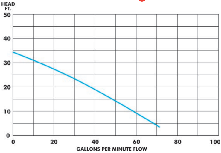
PX400 Performance Curve 2" Discharge
