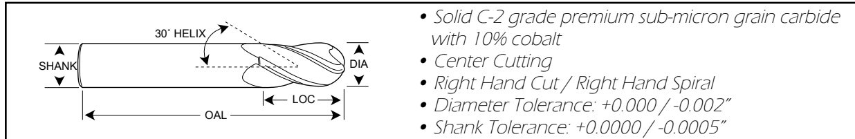
4 flute geometry offers increased core strength
