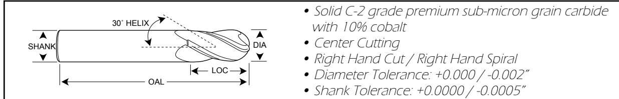
4 flute geometry offers increased core strength
