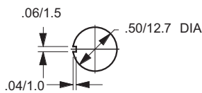
Mounting Hole With Keyway
