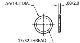
Knurled Nut
