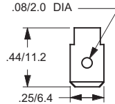
1/4" Q.C. Terminal
