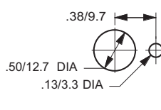
Mounting Hole With Locking Ring
