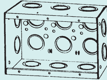
M3-250 5-7/16" Wide, Welded Three gang
