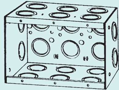
M3-350 5-7/16" Wide, Welded Three gang
