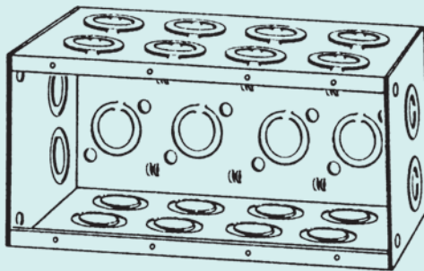
M4-350 7-3/8" Wide, Welded Four gang
