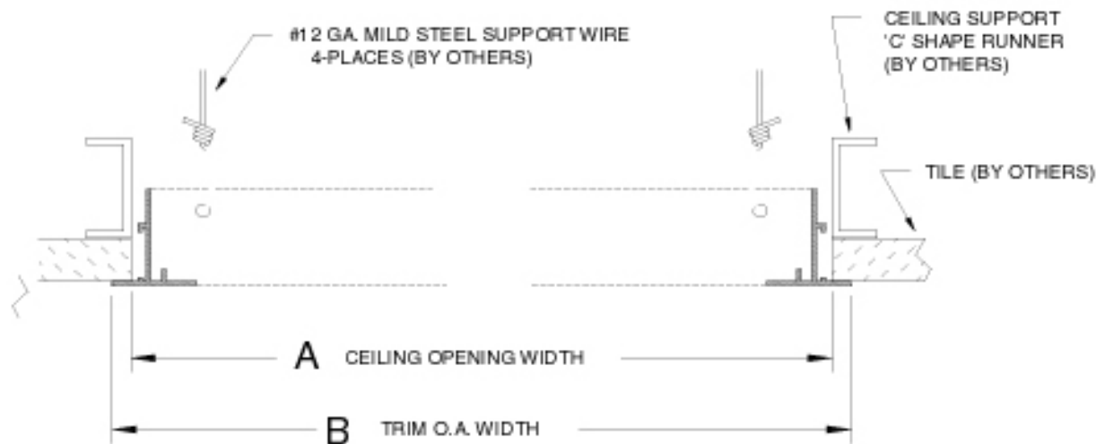
CROSS SECTION
