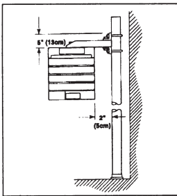
Pole Mounting Bracket
