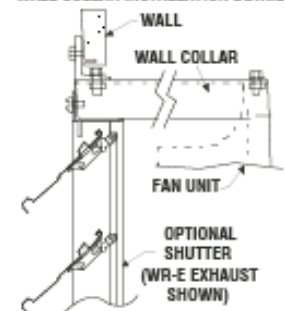
WALL COLLAR INSTALLATION DETAIL
