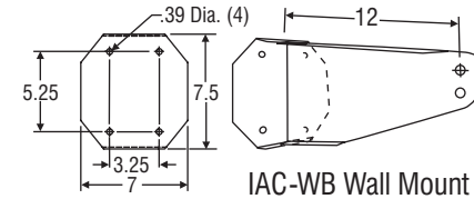
IAC-WB Wall Mount
