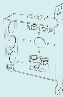
4SXVB-EK-PL 1-1/2" Deep, Welded Plain vertical bracket
