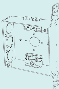
4SXAB-EK 1-1/2" Deep, Welded Vertical bracket with barbed hooks
