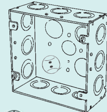
4SJD-EK 2-1/8" Deep, Welded
