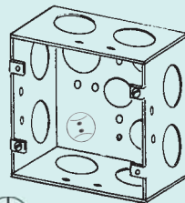
4SJD-1 2-1/8" Deep, Welded
