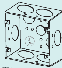
4SJD-1-1/4 2-1/8" Deep, Welded
