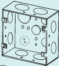
4SJ-3/4 1-1/2" Deep, Welded
