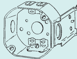
561LDJB 2-1/8" Deep JB bracket set back 1" Gauging notches set back 1-3/8" & 1-1/2"
