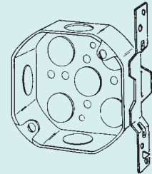
40VB-1/2 1-1/2" Deep Vertical bracket set back 5/8"
