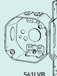
561LVB 1-1/2" Deep Plain vertical bracket set back 5/8"
