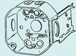
551LDJB 2-1/8" Deep JB bracket set flush, Gauging Notches 1-3/8" & 1-1/2"
