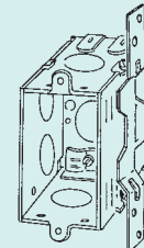
384D-VBPL 3-1/2" Deep, Gangable Plain vertical bracket set back 3/4"
