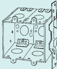
384VB-PL2G 2-1/2" Deep, Welded Plain vertical bracket set back 3/4"
