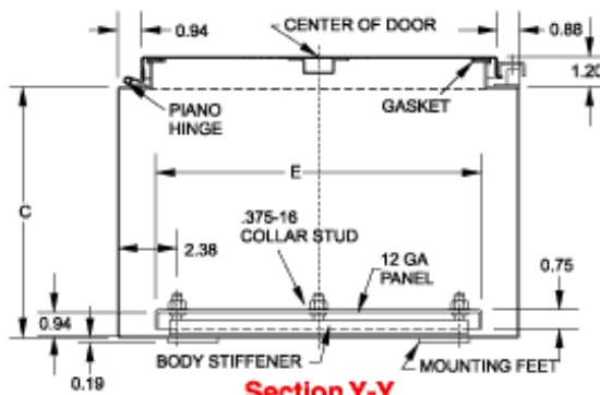
Section Y-Y
